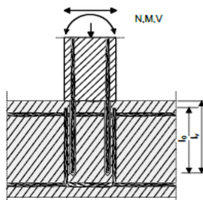
Figure 1.3 Overlap joint at a foundation of a column or wall where the rebar is stressed in tension
