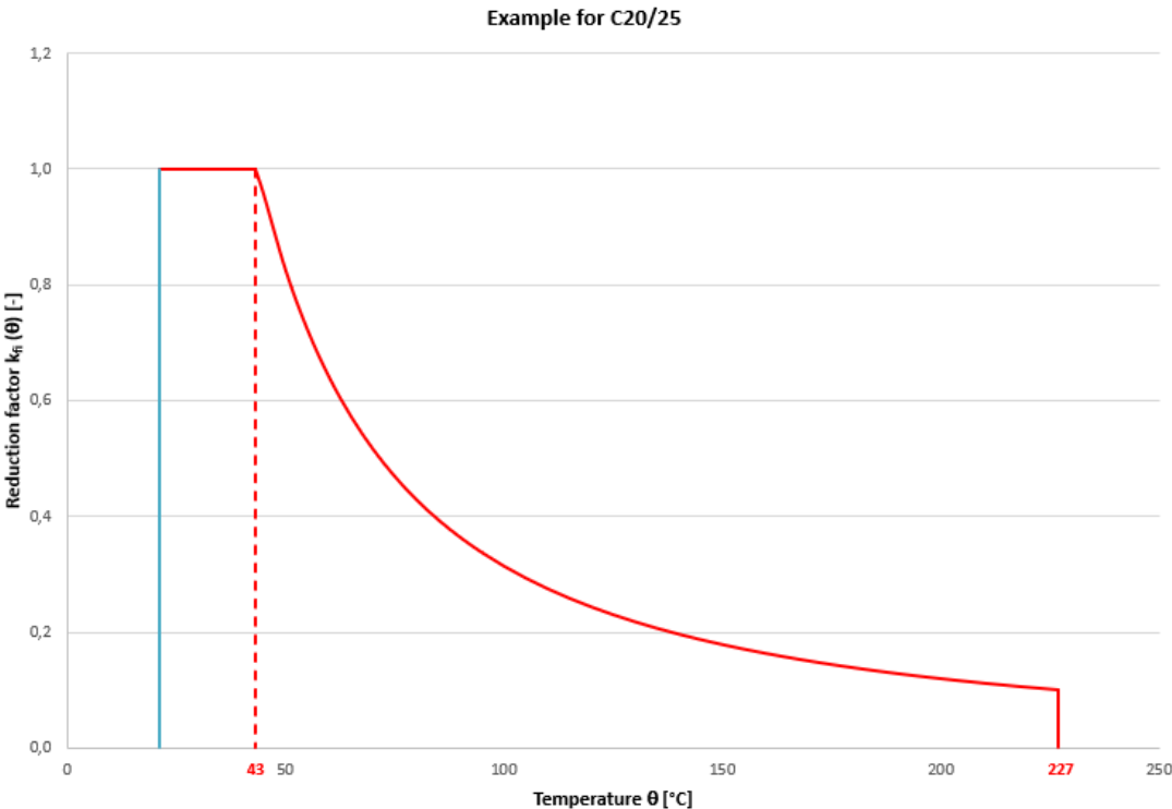
Figure C1: Example graph of Reduction factor k_{fi}(\theta) = k_{fi,100y}(\theta) for concrete classes C20/25 for good bond conditions for 50 and 100 years:
