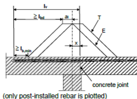
Figure 1.4 End anchoring of slabs or beams, designed as simply supported
